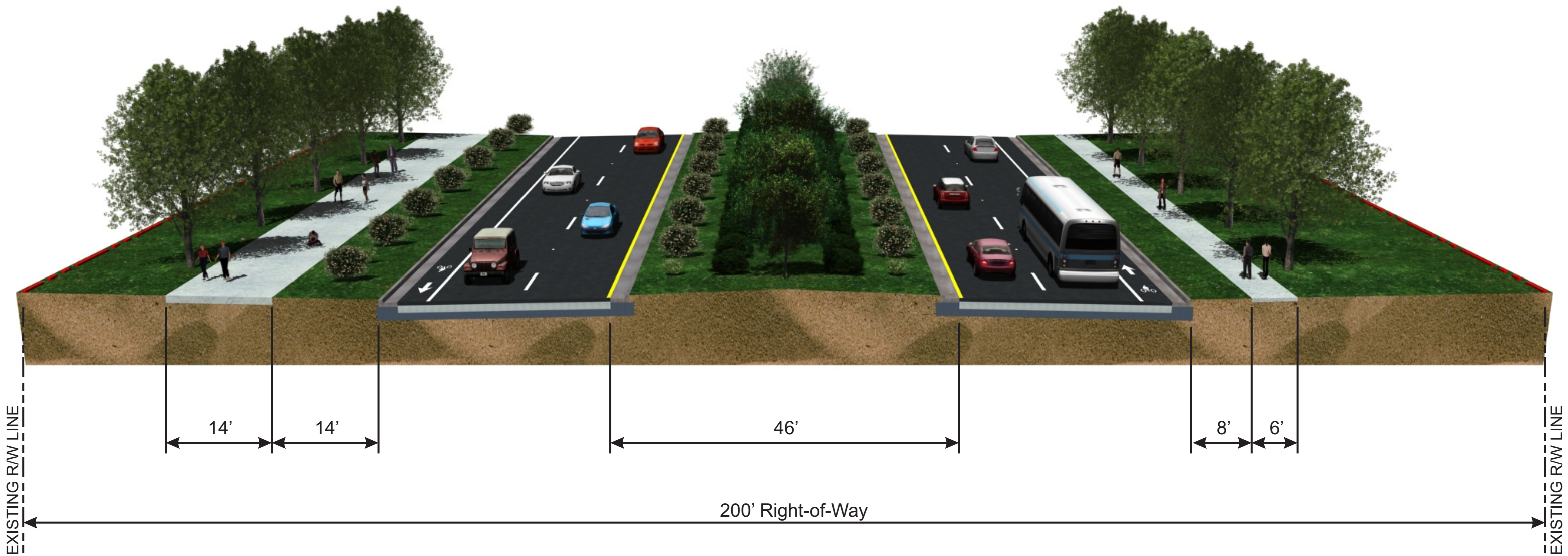
Peters Creek Parkway (NC 150) Typical Roadway Section - 200' Right-of-Way From Silas Creek Parkway to 1600' South of Academy Street
